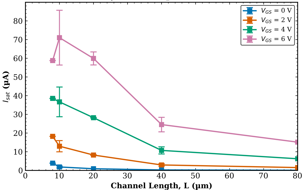
TFT3 Combined (Tr. 1 & 2) I_{sat} vs L | W = 100 \mu\text{m} (mean \pm std)
